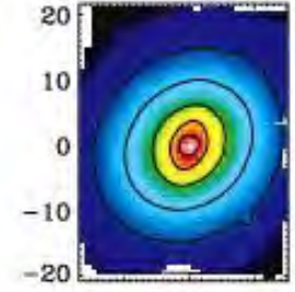
NGC 2699 ↖
