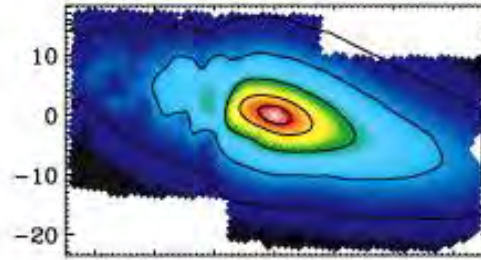
NGC 2685 ↖
