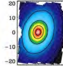
NGC 2695 ↗
