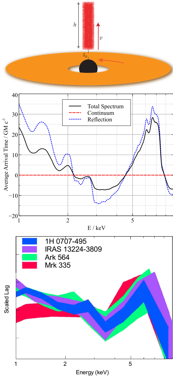
Fig. 5 Top: Schematic model of vertically extended corona in which the matter flows upward at velocity v (Wilkins et al. 2016). Centre: Lag energy spectrum resulting from this model when v increases upward with height h . Lower: Lag energy spectrum for 4 objects in which the dip at 3–4 keV matches that seen in the centre panel.
