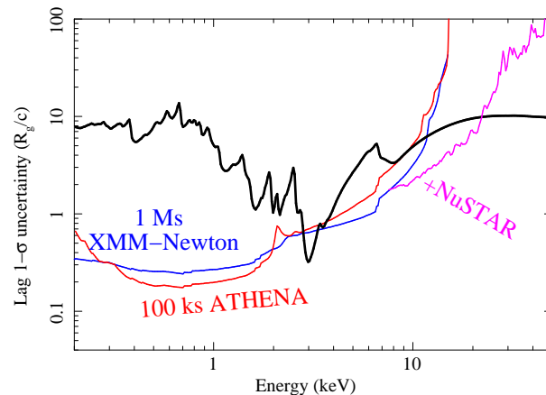
Fig. 4 Simulation showing achievable sensitivity in units of r_g/c , adapted from (Uttley et al. 2014). The black line is a ‘sample’ lag-energy spectrum (for a 10^6 M_\odot AGN). The assumed 2–10 keV flux is 4 \times 10^{-11} cgs (for AGN everything scales with \sqrt{\text{flux}} so it is easy to see what is needed for other flux levels). The lag errors just scale with 1/\sqrt{\text{exposure time}} . Note that whilst a 100 ks ATHENA exposure can statistically match a 1 Ms XMM-Newton exposure on high frequency lags (modelled here) it cannot reach the lowest frequency propagation lags ( \ll 10^{-4} ). Similarly, the long XMM-Newton exposures yield an average result whereas a shorter ATHENA exposure can follow the changes in a corona on 100 ks timescales.
