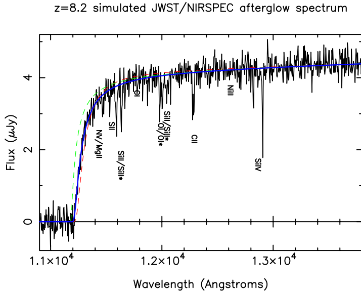
Figure 12: Simulated JWST /NIRSPEC spectrum of a GRB afterglow based on GRB090423, as it would have been observed 4 days post-burst in a 5 hr exposure. This clearly shows that high S/N spectroscopy will be possible even for faint afterglows using JWST . The simulation assumed a 100% neutral IGM and a host HI column density of \log(N_{\text{H}}/\text{cm}^{-2}) = 21 . The continuum cannot be fit by either a pure neutral IGM model (green line), or a pure host model with an ionized IGM (red line). Instead the two components can be decomposed, as illustrated with the blue fit.
