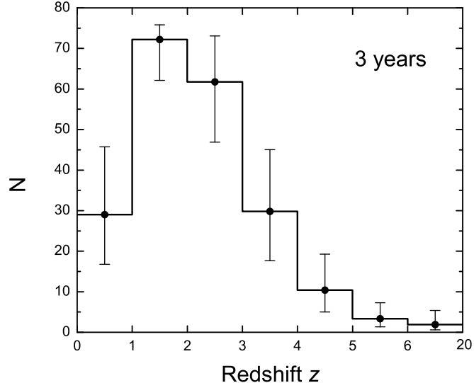
Figure 11: Simulated redshift distribution of GRBs to be detected by ECLAIRs during the 3 year mission lifetime. Error bars show the 2\sigma uncertainties of the assumptions on the GRB population (i.e., the 2\sigma uncertainties of the GRB rate density evolution, \delta = 1.7 \pm 2\sigma ) in the redshift bin.
