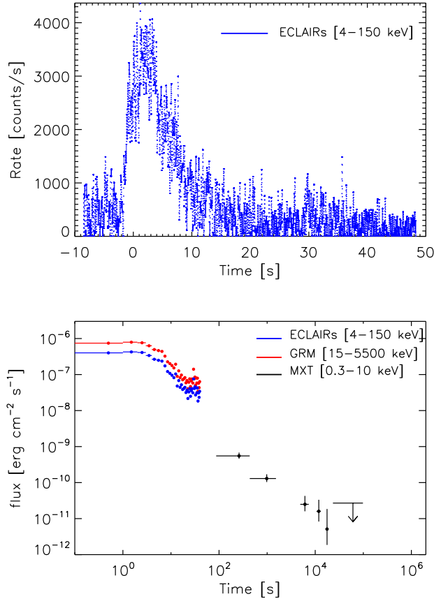
Figure 7: Simulation of the prompt and afterglow emission of a long GRB in SVOM instruments. GRB 091020 is a classical long GRB detected by Swift and Fermi /GBM. Using GBM data (Gruber et al., 2014b) for the prompt emission and Swift /XRT data for the X-ray afterglow (Evans et al., 2007, 2009), this GRB has been simulated in ECLAIRs and GRM, assuming that the GRB is on-axis for ECLAIRs and therefore 30^\circ off-axis in GRM, and in MXT where the afterglow is detected up to \sim 10^4 s. Left : simulated prompt light curve in counts per seconds in ECLAIRs. Right : prompt and afterglow flux in log-log scale simulated in ECLAIRs, GRM and MXT.
