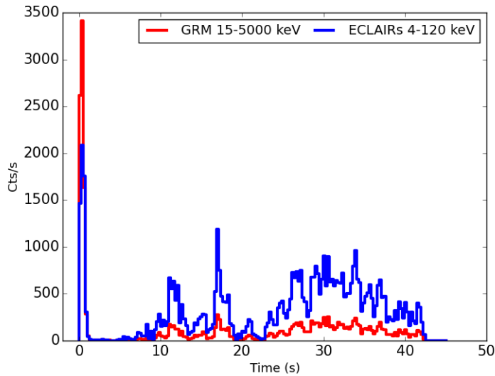
Figure 10: Simulation of the light curve of a short GRB with a soft extended emission in SVOM /ECLAIRs+GRM. GRB 990712A shows an initial short and hard spike, leading to the classification as a short hard GRB, followed by a soft extended emission (Norris & Bonnell, 2006). The simulated light curve is plotted in counts per second in ECLAIRs and GRM, based on the time-dependent spectral analysis published by Kaneko et al. (2006a) and assuming that the GRB is on-axis for ECLAIRs and therefore 30 off-axis in GRM. During the initial hard spike, GRM is more sensitive than ECLAIRs: it is detected at 62\sigma in GRM and 41\sigma in ECLAIRs. Therefore, in the case of weaker short GRBs, the detection by GRM may be used to increase confidence in a marginal ECLAIRs detection and to lower the slew threshold. During the soft extended emission, ECLAIRs becomes more sensitive: detection at 77\sigma in ECLAIRs and 15\sigma in GRM. Therefore the combination of the two instruments will allow to increase the sensitivity of SVOM to short GRBs and the capacity to slew and catch their early afterglow.
