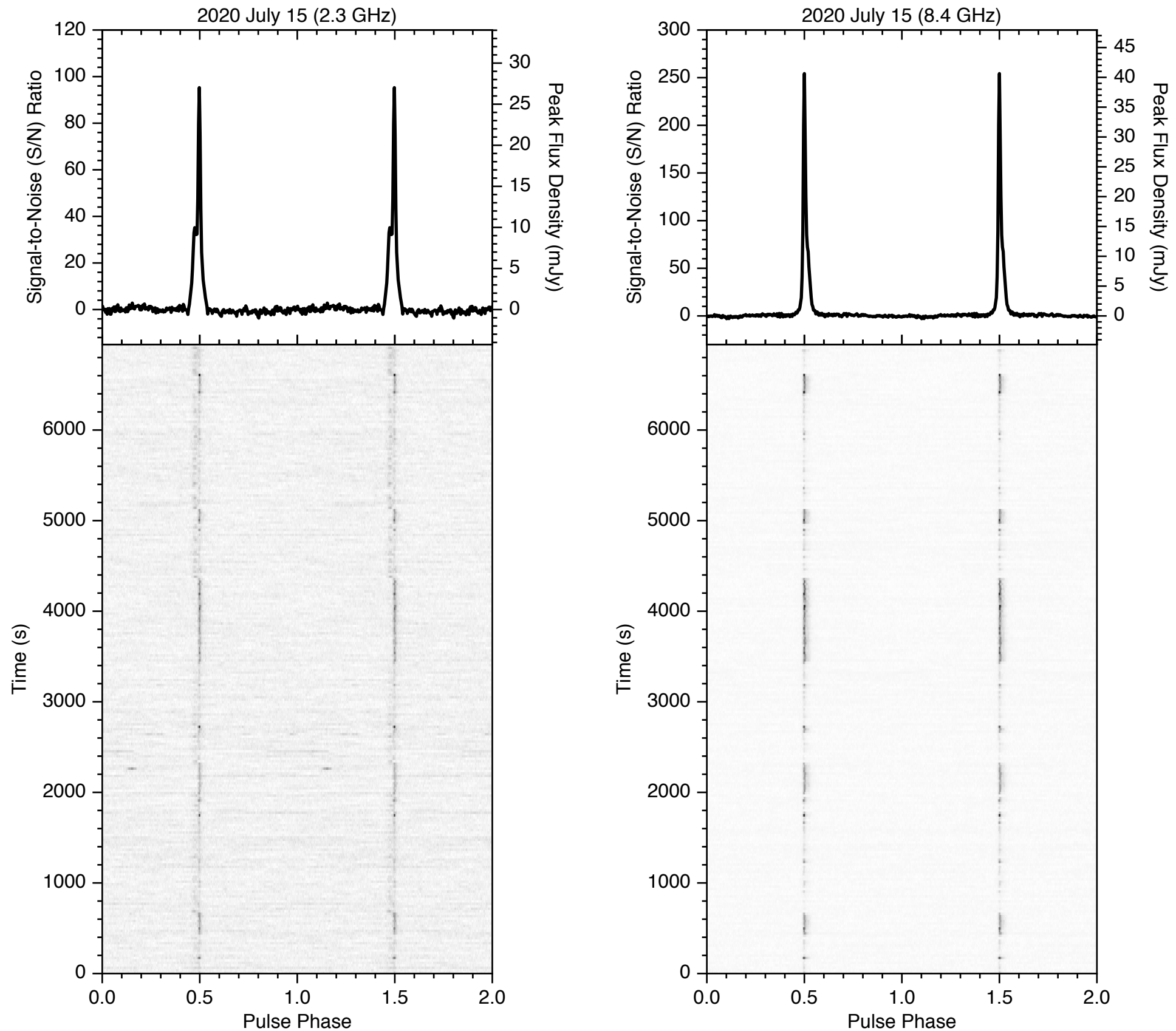
Figure 1: Dynamic spectra of Swift J1818.0-1607's pulsed radio emission, detected on 2020 July 15 at both S-band (left panels) and X-band (right panels) using DSS-63 in Madrid, Spain. The top panels show the integrated pulse profiles at each frequency band, while the bottom panels show the temporal behavior of the pulse profiles over the \sim 2.1 hour observation.
