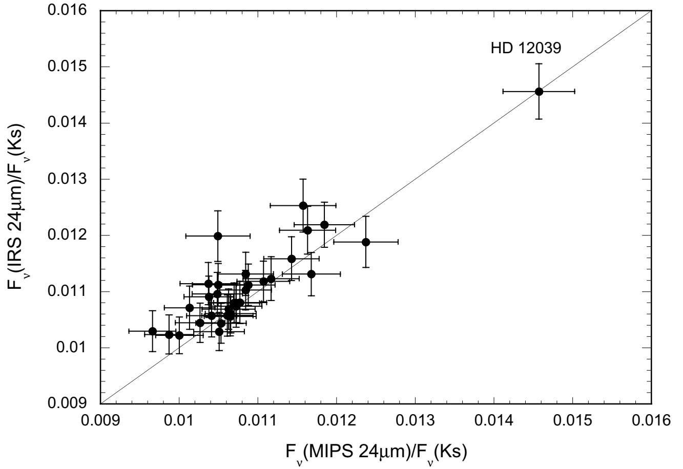
Fig. 2.— The F_{\nu}(24\mu\text{m})/F_{\nu}(\text{Ks}) ratio for measurements from IRS & MIPS for the 33 stars in the FEPS V1.1 data release. HD 12039 stands out clearly as having an anomalously high F_{\nu}(24\mu\text{m})/F_{\nu}(\text{Ks}) ratio in both instruments indicating a significant 24\mu\text{m} excess above the photosphere. The solid line is of slope = 1.
