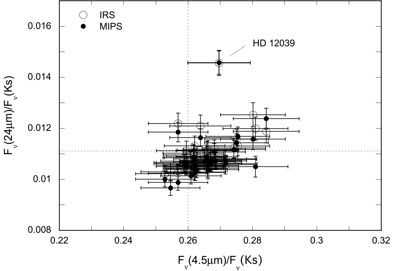
Fig. 1.— Flux ratio diagram [ F_{\nu}(24\mu\text{m})/F_{\nu}(\text{Ks}) vs. F_{\nu}(4.5\mu\text{m})/F_{\nu}(\text{Ks}) ] for the 33 stars in the FEPS V1.1 data release. Data are shown from both the MIPS 24\mu\text{m} broad band photometry and from a synthetic broad band point centered at 24\mu\text{m} formed from the IRS spectra. Note that the F_{\nu}(4.5\mu\text{m})/F_{\nu}(\text{Ks}) ratio for HD 12039 is near the median for the other 32 stars consistent with photospheric colors, but the F_{\nu}(24\mu\text{m})/F_{\nu}(\text{Ks}) ratio is anomalously high indicating a significant 24\mu\text{m} excess above the photosphere. Error bars represent 1\sigma in the ratios calculated from the internal IRS and MIPS measurement uncertainties, and the total uncertainties of the 2MASS K_s flux densities. The 24\mu\text{m} excess from HD 12039 is detected in both MIPS and IRS independently and at different epochs. The dotted lines indicate the ratios predicted by the best-fit Kurucz model atmosphere for HD 12039. Stars with photospheric temperatures different than HD 12039 will have slightly different F_{\nu}(4.5\mu\text{m})/F_{\nu}(\text{Ks}) ratios, which explains the dispersion in this quantity for the 33 stars in the sample.
