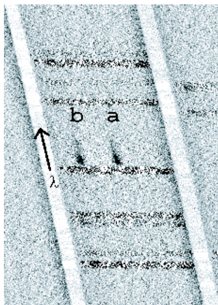
Figure 3: Confirmation of strong emission in the pair of images marked in Figure 1 using the Keck II Echelle Spectrograph and Imager. (a) 2-D sky subtracted spectral image using the 20 arcsec slit. (b) Flux-calibrated spectrum of the region around Lyman alpha emission combined from both images revealing a P-Cygni like profile extending redward by \simeq 200 km sec ^{-1} in the rest-frame. The redshift corresponding to the peak emission is z=5.576 .
