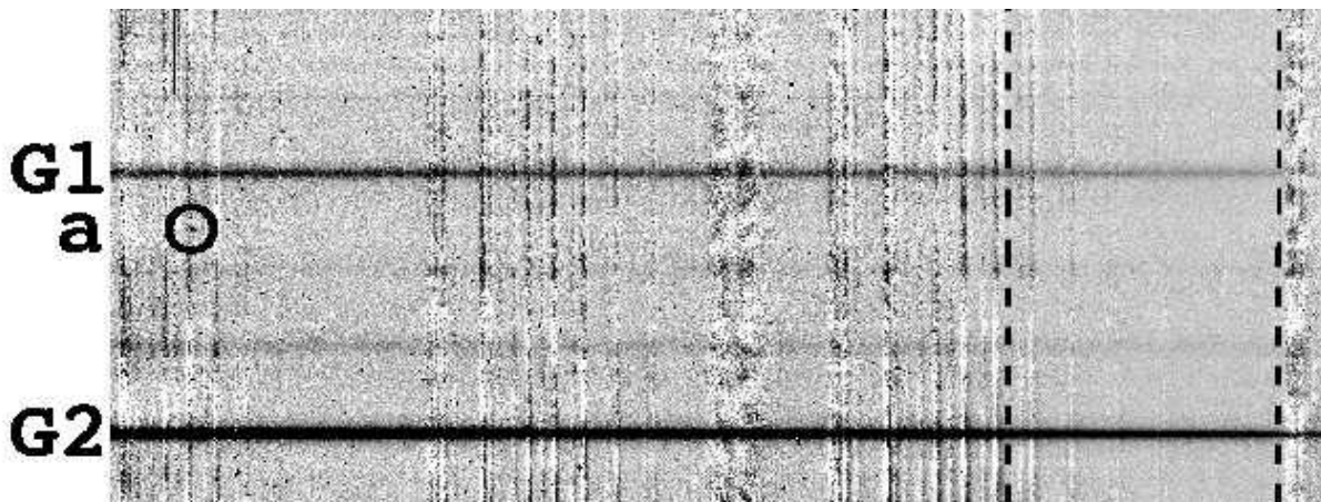
Figure 2: The discovery of an emission line source close to the cD in the rich cluster Abell 2218. Keck I LRIS-R spectral image of a region 100 arcsec in extent covering \lambda\lambda 6700-9350 Å with the emission line attributed to object a at \lambda 7989 Å marked. The dashed lines at longer wavelengths refer to the wavelength range used to deduce a statistical upper limit on a stellar continuum from the source (see text). The spectra of fiducial cluster galaxies G1 and G2 labelled in Figure 1 are marked.
