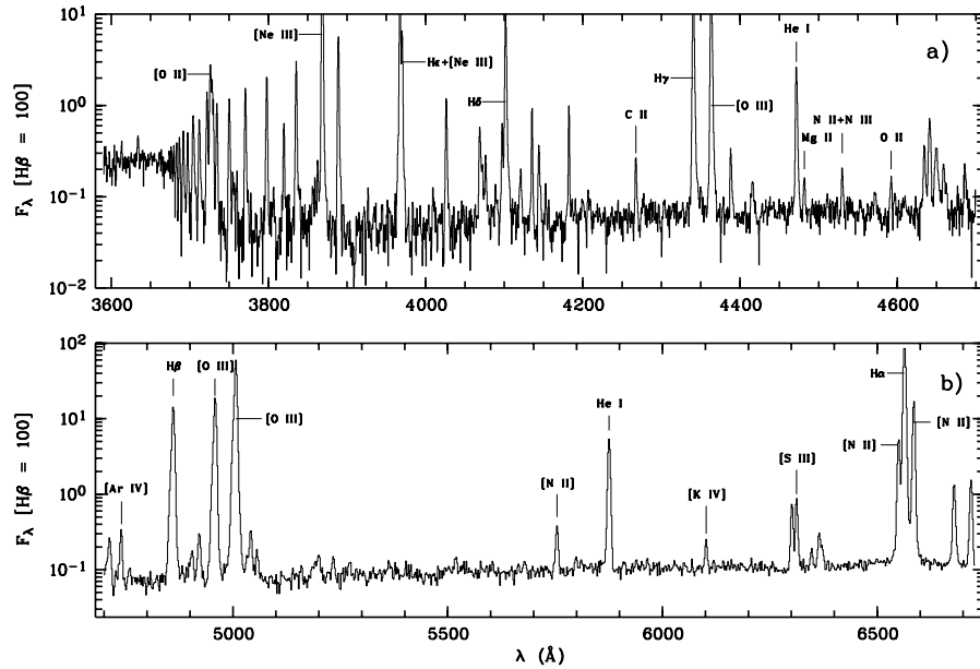
Fig. 1. Optical spectrum of M2-24 from a) 3600–4700 Å and b) 4700–6700 Å. Note that H \alpha and [O III] \lambda 5007 were saturated in this exposure. Interstellar extinction has not been corrected for.
