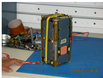
Stack with simulated solar panels and X-Band patch. Pre-deployed VHF/UHF antennas.
