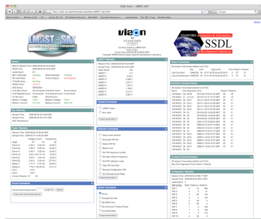
Web-based Telemetry Display
