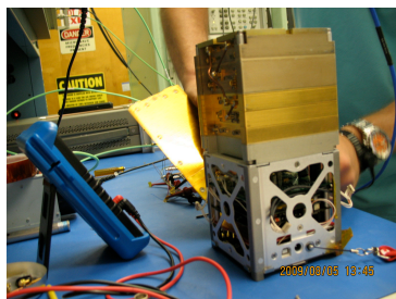
Stacked Cubesat bus and LMRST
