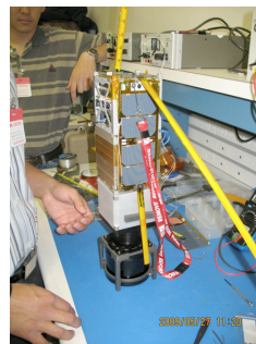
Satellite during command / telemetry demonstration with antennas deployed.
