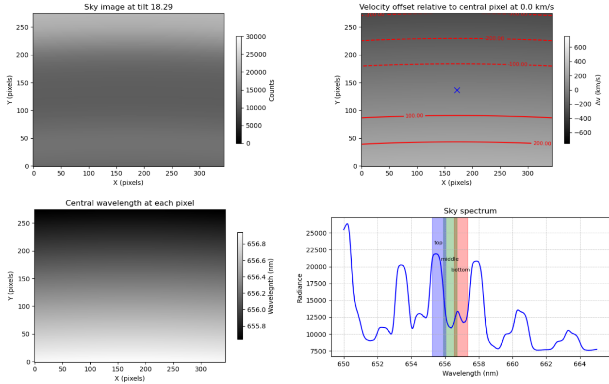
Figure 22. Same as Figure 21 but where the filter tilt (angle of the surface normal of the filter with respect to the optical axis) is 18.29°.
