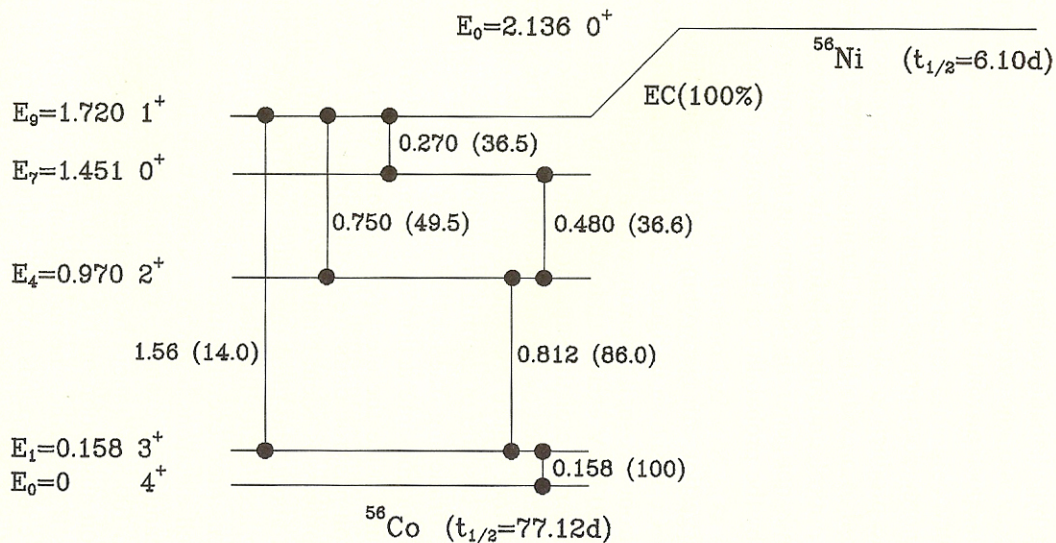
Fig. 13.3. Simplified ^{56}\text{Ni} Decay
