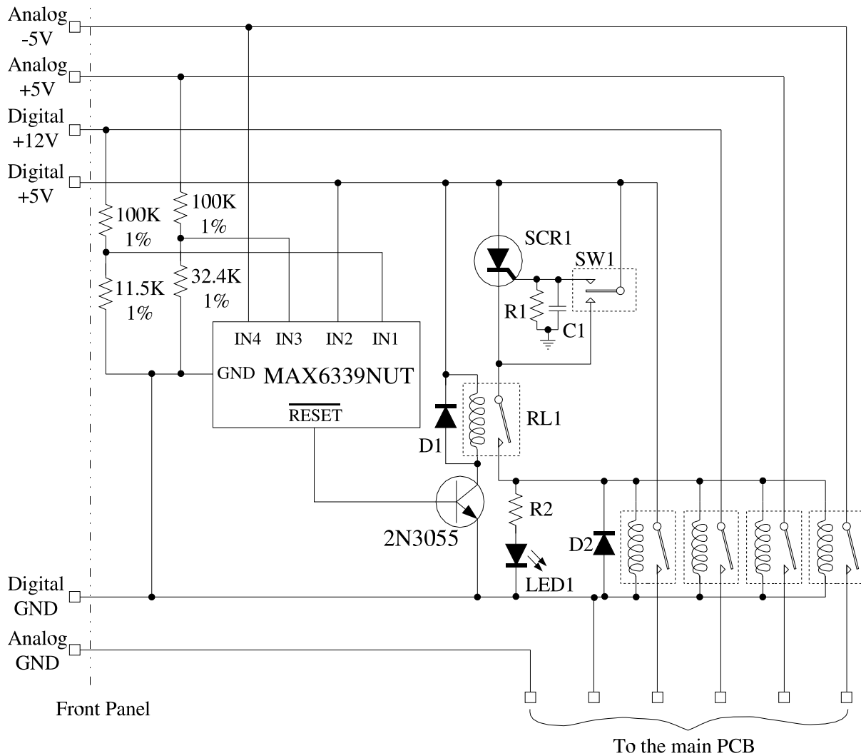
Figure 3.3: The power-management circuit and its front-panel power switch
